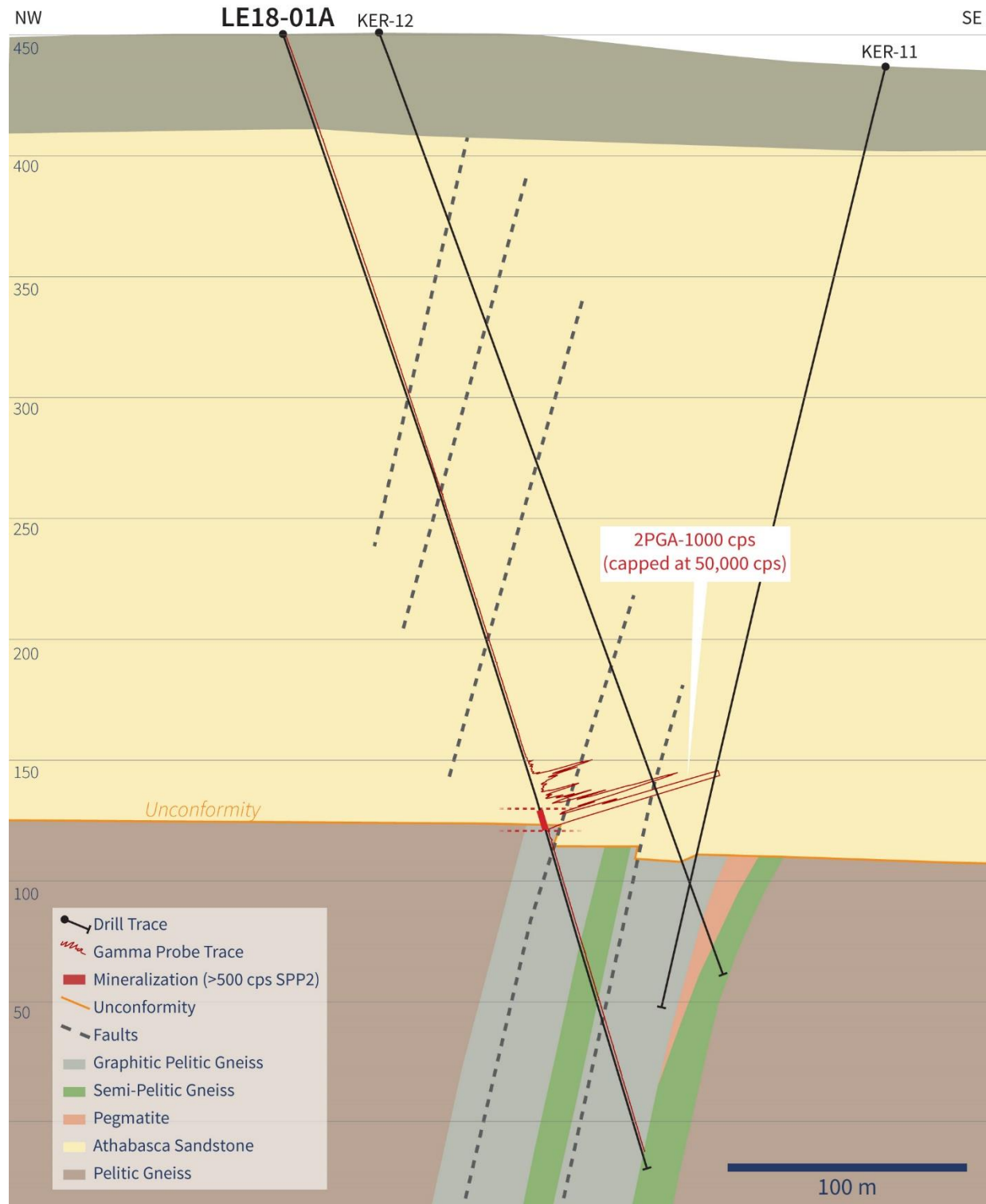
Figure 2 – Cross-Section Through Drill Hole LE18-01A
